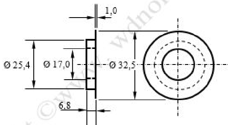
Hub Bearing Oil Retaining Felt Washer, Steel Cup Off-side (Front or Rear) p/n 3741
