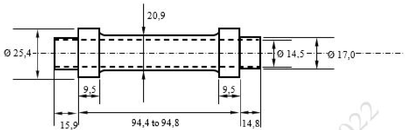
Hub Shell Bearing Sleeve front and rear p/n 9491
